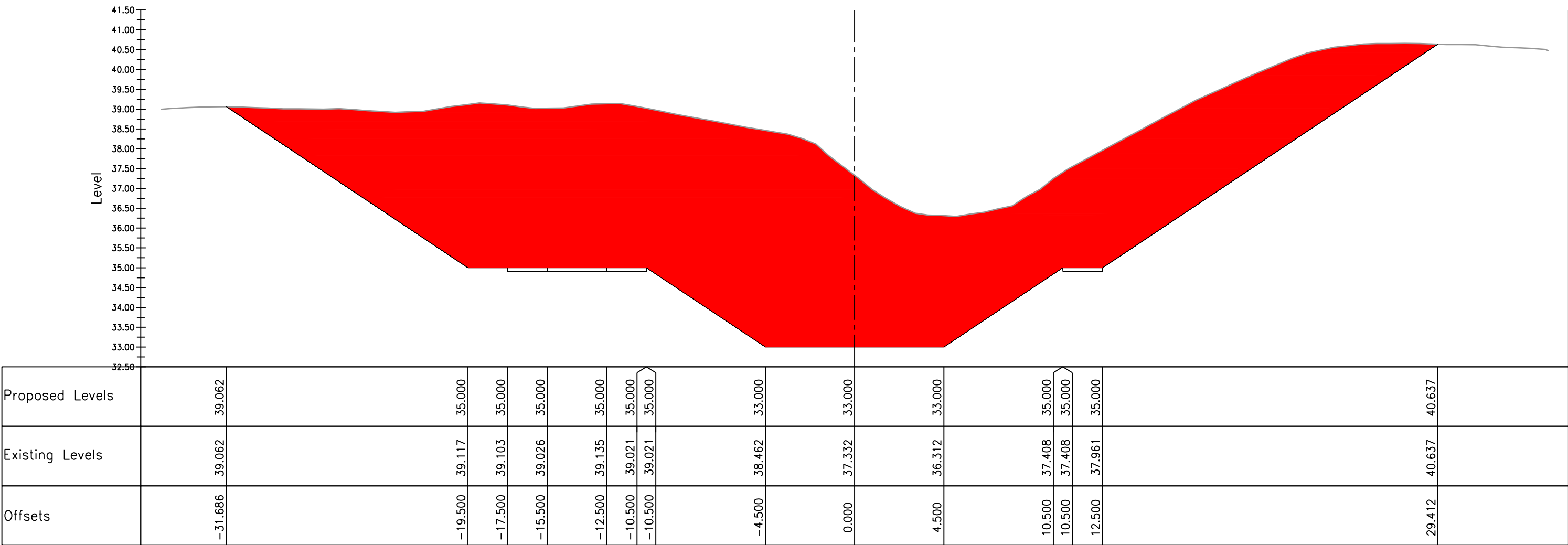
BMK section M to Q Ch. 150.000, Horiz. 1:200, Vert. 1:100
