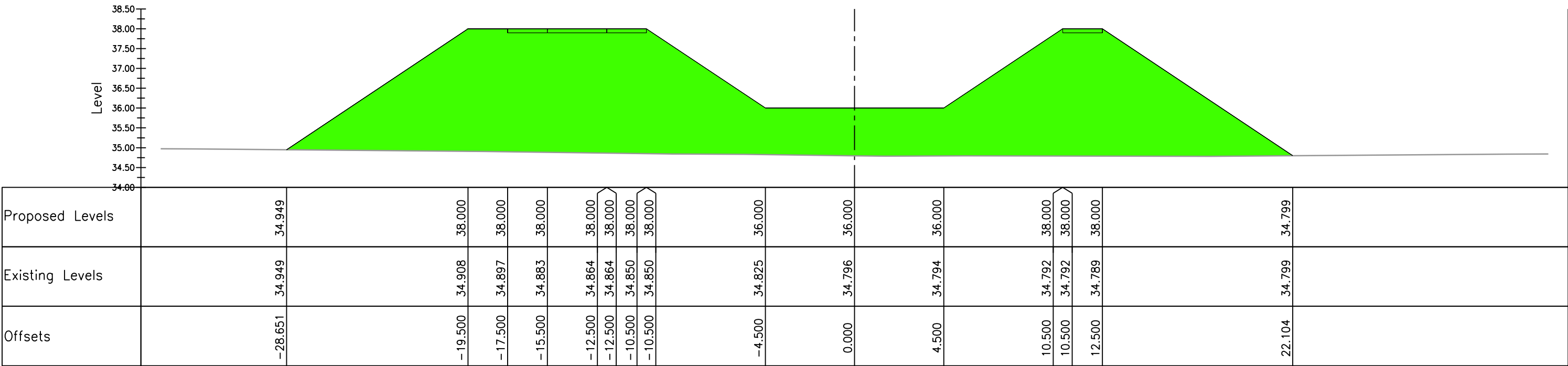
BMK section M to Q Ch. 1300.000, Horiz. 1:200, Vert. 1:100
