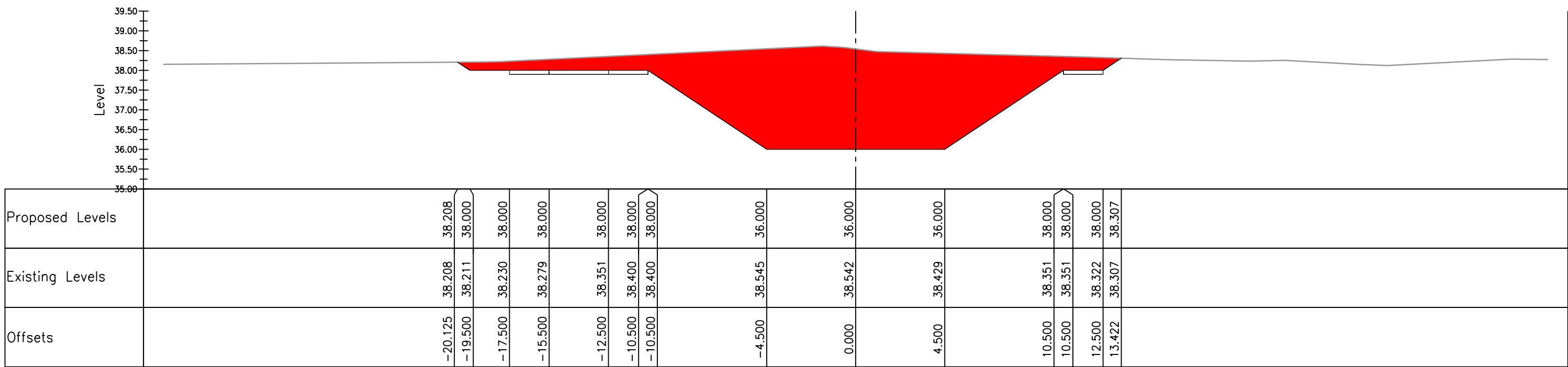
BMK section M to Q Ch. 1000.000, Horiz. 1:200, Vert. 1:100
