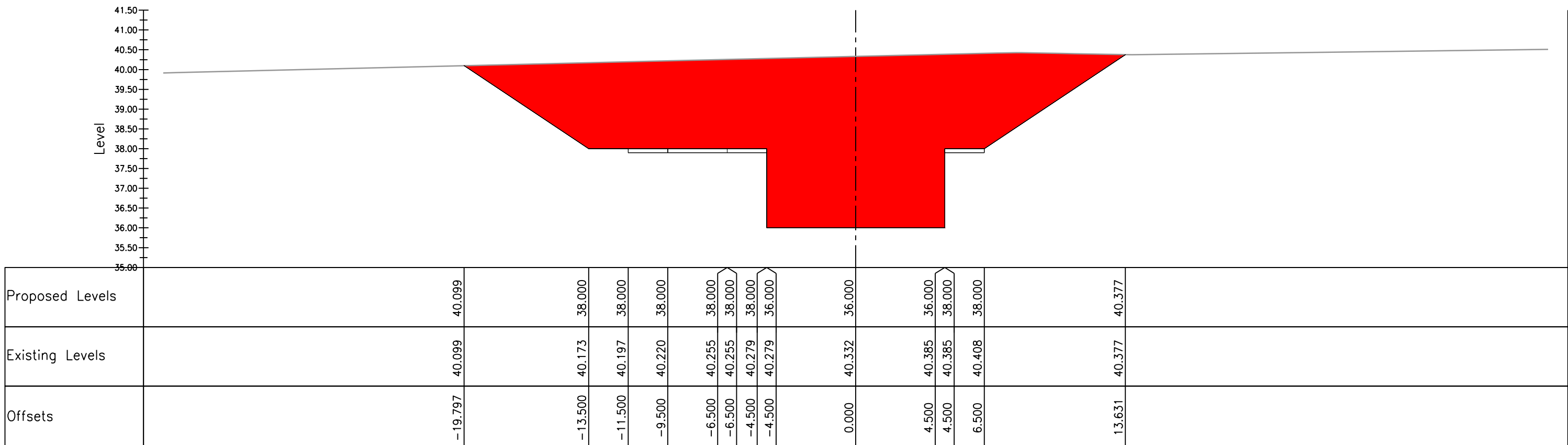
BMK section M to Q Ch. 850.000, Horiz. 1:200, Vert. 1:100
