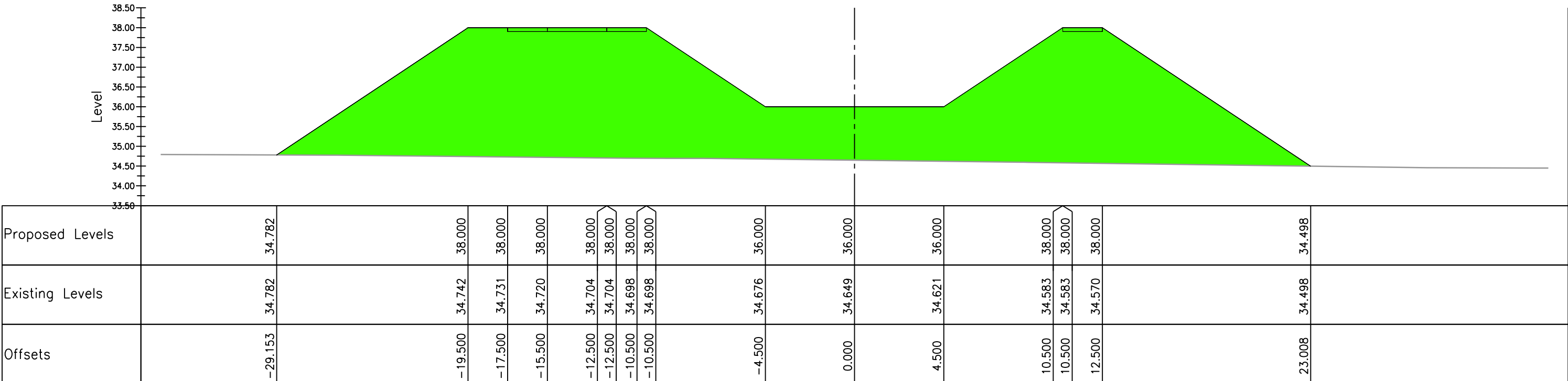
BMK section M to Q Ch. 1350.000, Horiz. 1:200, Vert. 1:100
