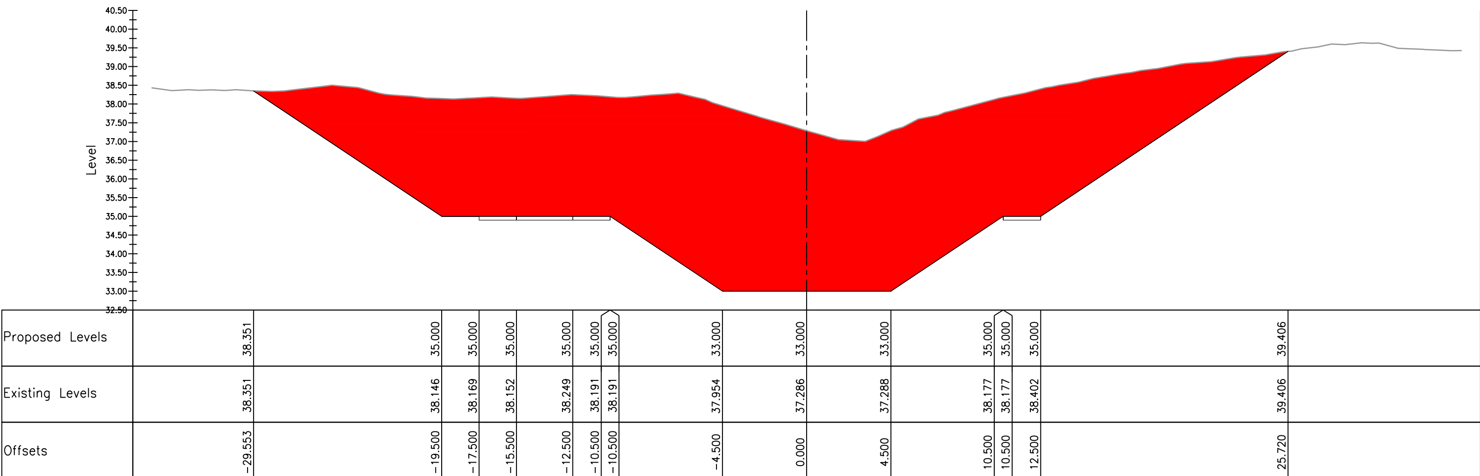
BMK section M to Q Ch. 250.000, Horiz. 1:200, Vert. 1:100
