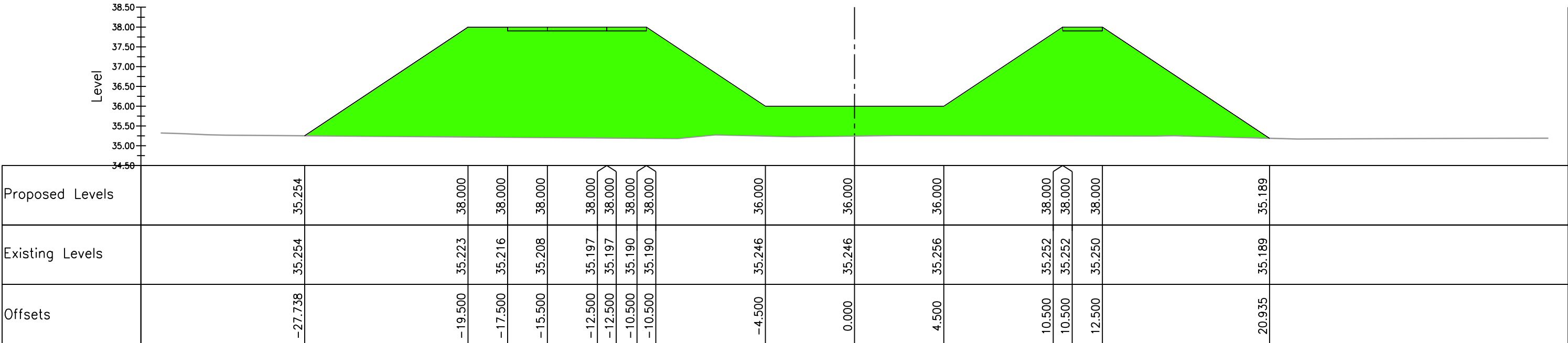
BMK section M to Q Ch. 1250.000, Horiz. 1:200, Vert. 1:100
