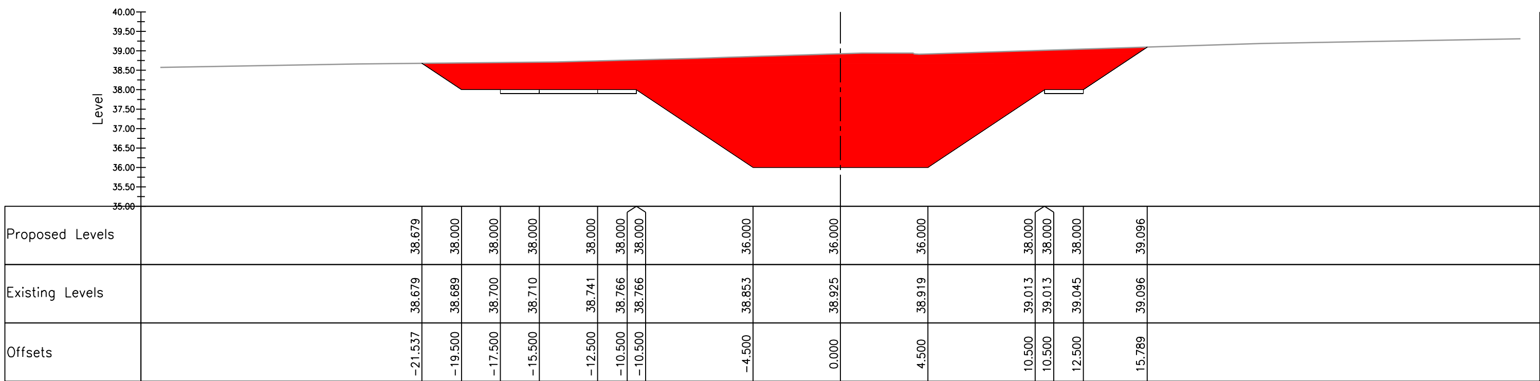
BMK section M to Q Ch. 950.000, Horiz. 1:200, Vert. 1:100
