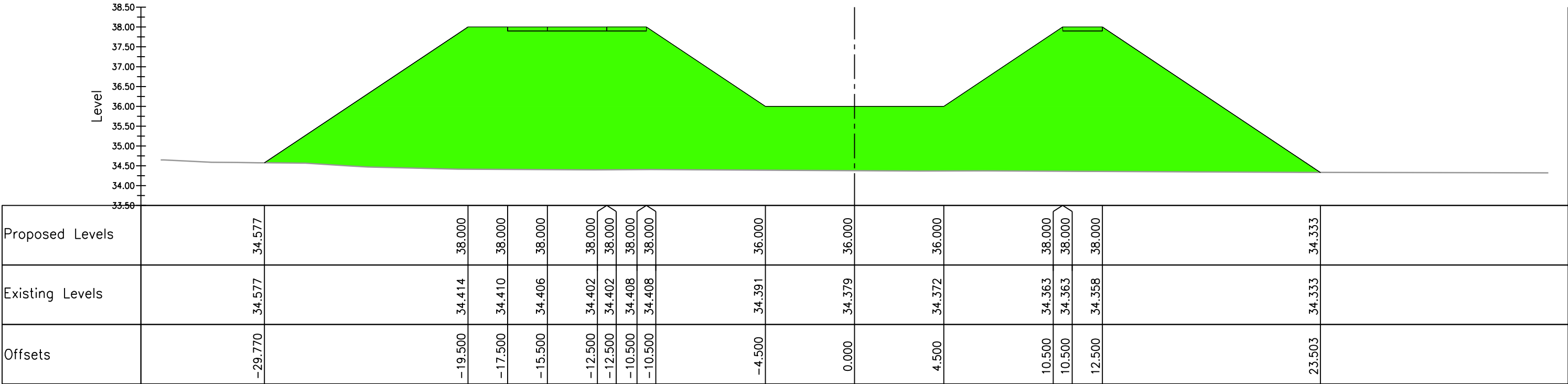
BMK section M to Q Ch. 1400.000, Horiz. 1:200, Vert. 1:100
