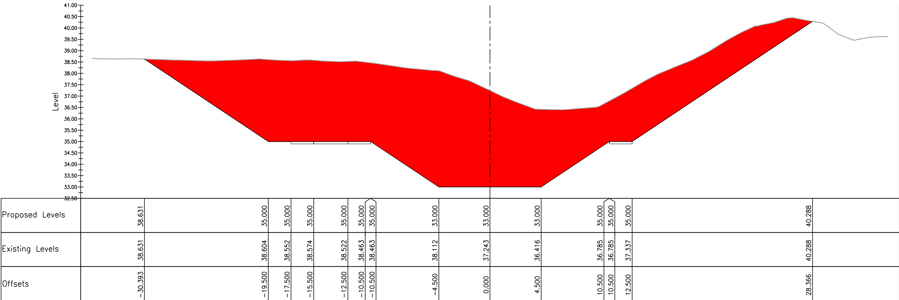
BMK section M to Q Ch. 200.000, Horiz. 1:200, Vert. 1:100
