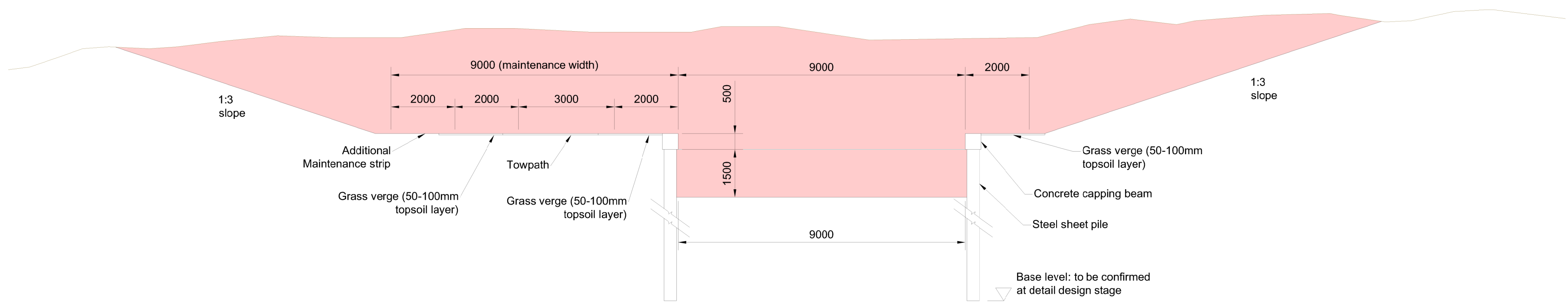
CUT ONLY SCALE 1:100 at A1
