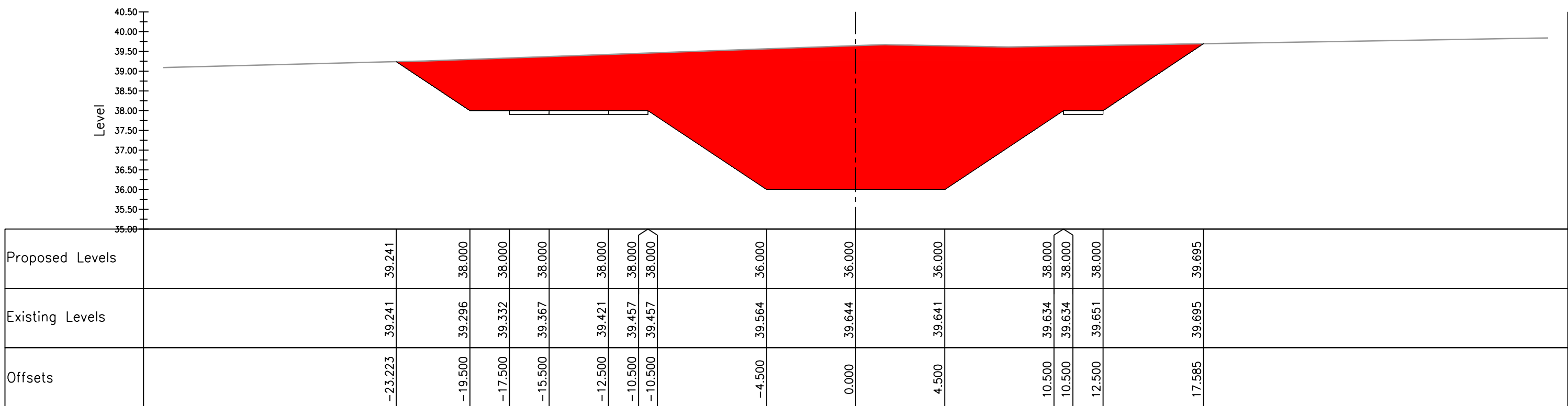
BMK section M to Q Ch. 900.000, Horiz. 1:200, Vert. 1:100
