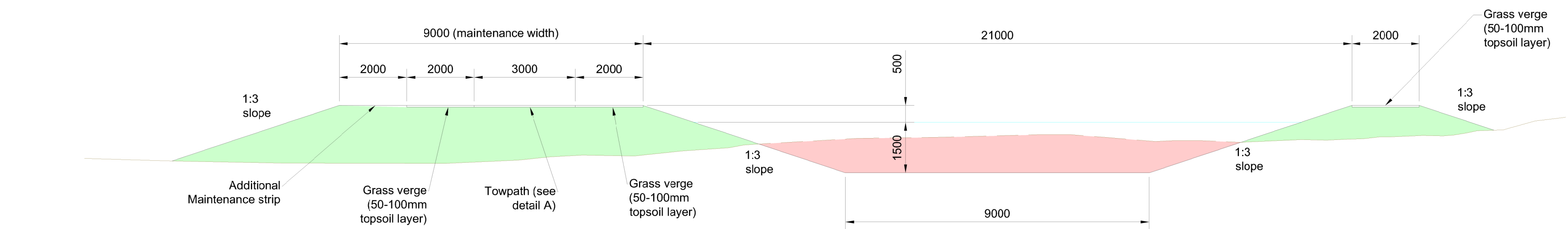
PARTIAL CUT AND FILL SCALE 1:100 at A1
